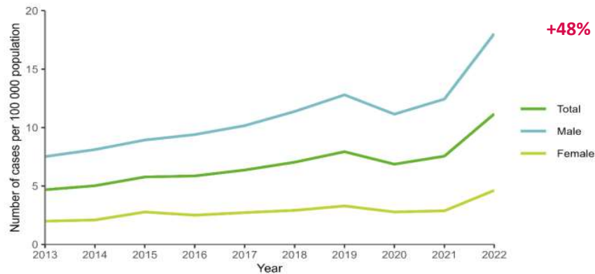
Figure 4. Notification rates of confirmed gonorrhoea cases per 100 000 population, total and by gender in EU/EEA countries reporting consistently, 2013-2022
